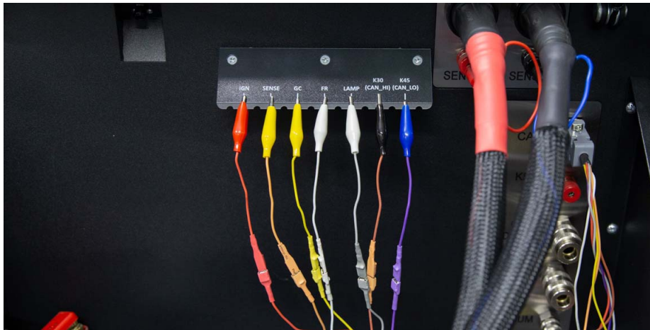
Figure 7. Diagnostic cable alligator clips that are set on the bracket.
