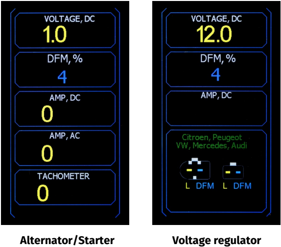
Figure 4. Bench display during the diagnostics of alternator/voltage regulator of type Lamp type or starter
